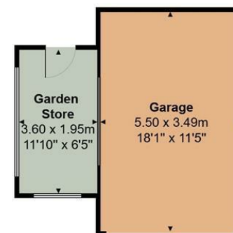
Lower Ground Floor Total Floor Area 26.5 m 2 ... 285 ft 2
